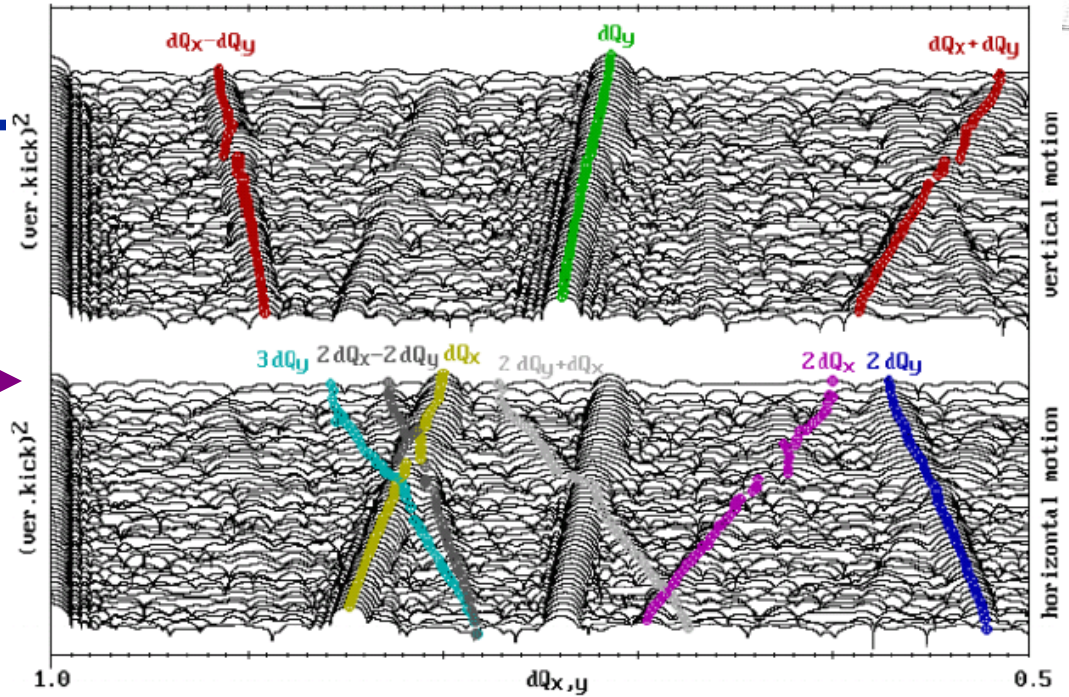
Figure 1: Spectra of the vertical and horizontal beam motion (top and bottom) with the fundamental tunes: dQ_x (yellow), dQ_y (green) and combinations of them.
